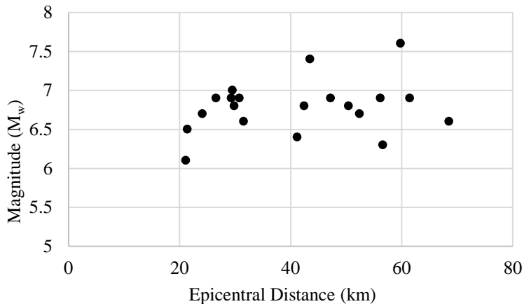
Figure 4 : Relationship of the ground motion record parameters
